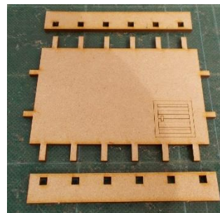
The base of the top floor and its supports.
