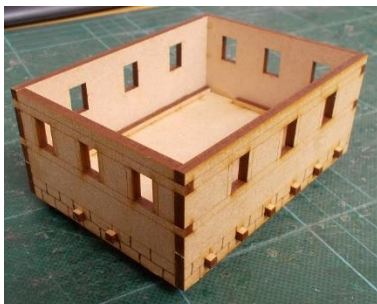
Glue the walls into place.
