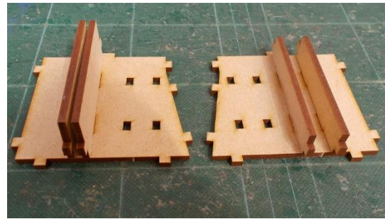
Glue the connectors to the main supports – the wider connectors being the ones closest together.
