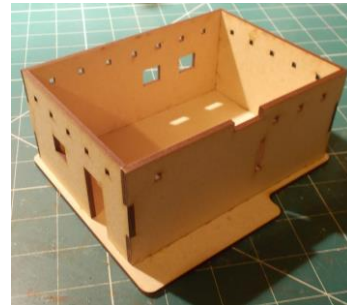
Glue them together as shown to form an open topped box.
