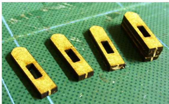
Each of the legs is formed from three pieces, glued together as shown.
