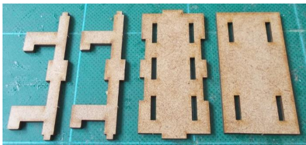
Each end of the wall is formed from the pieces shown above.
